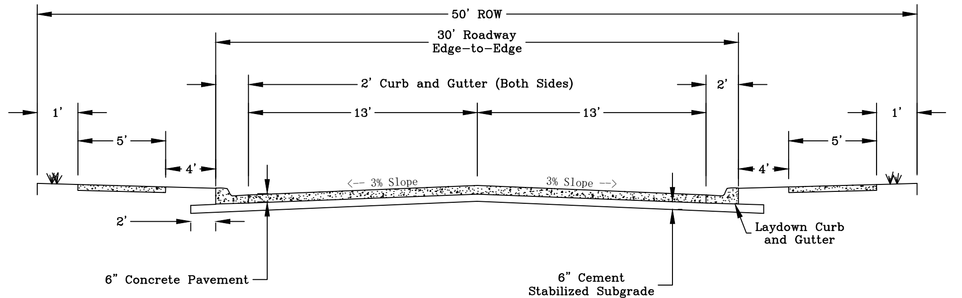
Typical Street & Utility Layout: N.T.S.
