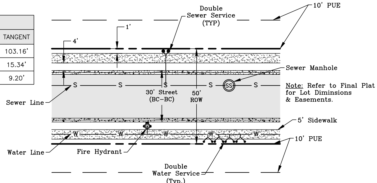
Typical Street & Utility Layout: N.T.S.
